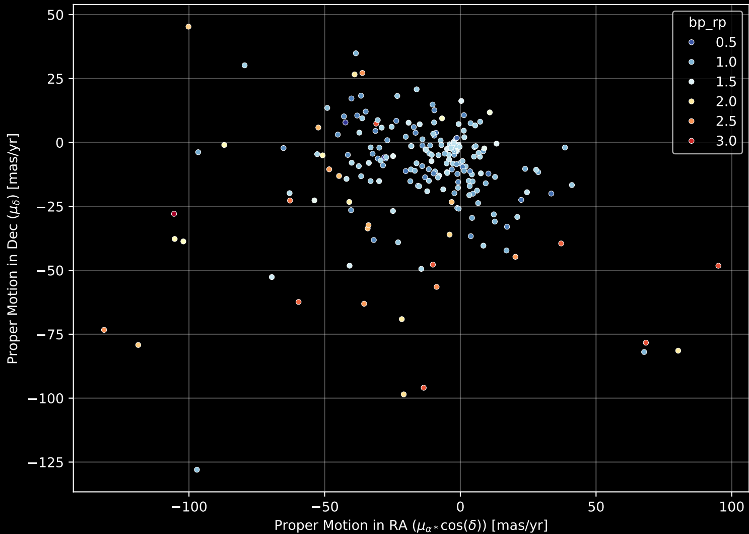
APOGEE DR17 Field: [K2_C14_251+55] Proper Motion Diagram (n= 211)
