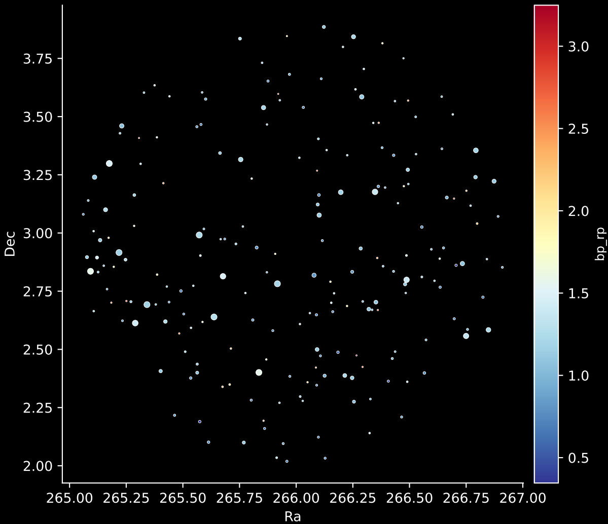
APOGEE DR17 Field: [K2_C14_251+55] Stars: 211
