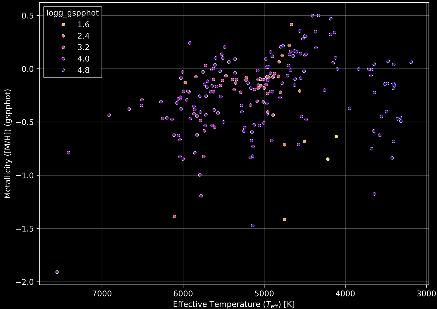
APOGEE DR17 Field: [K2_C14_251+55] Stellar Population Parameters (n= 211)
