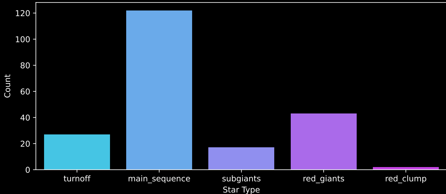
APOGEE DR17 Field: [K2_C14_251+55] Count plot of Star Type
