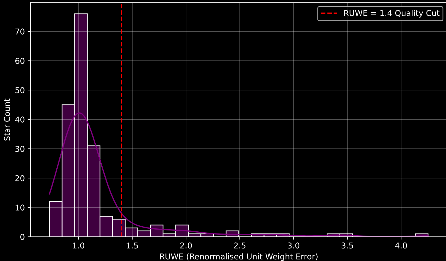
GAPOGEE DR17 Field [K2_C14_251+55] RUWE Distribution (n= 201)
