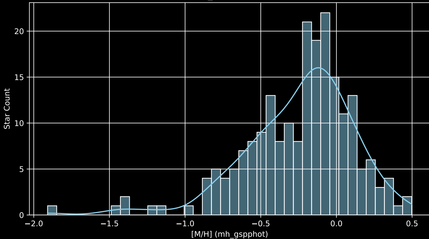
APOGEE DR17 Field: [K2_C14_251+55 [M/H] (mh_gspphot) (n= 210)
