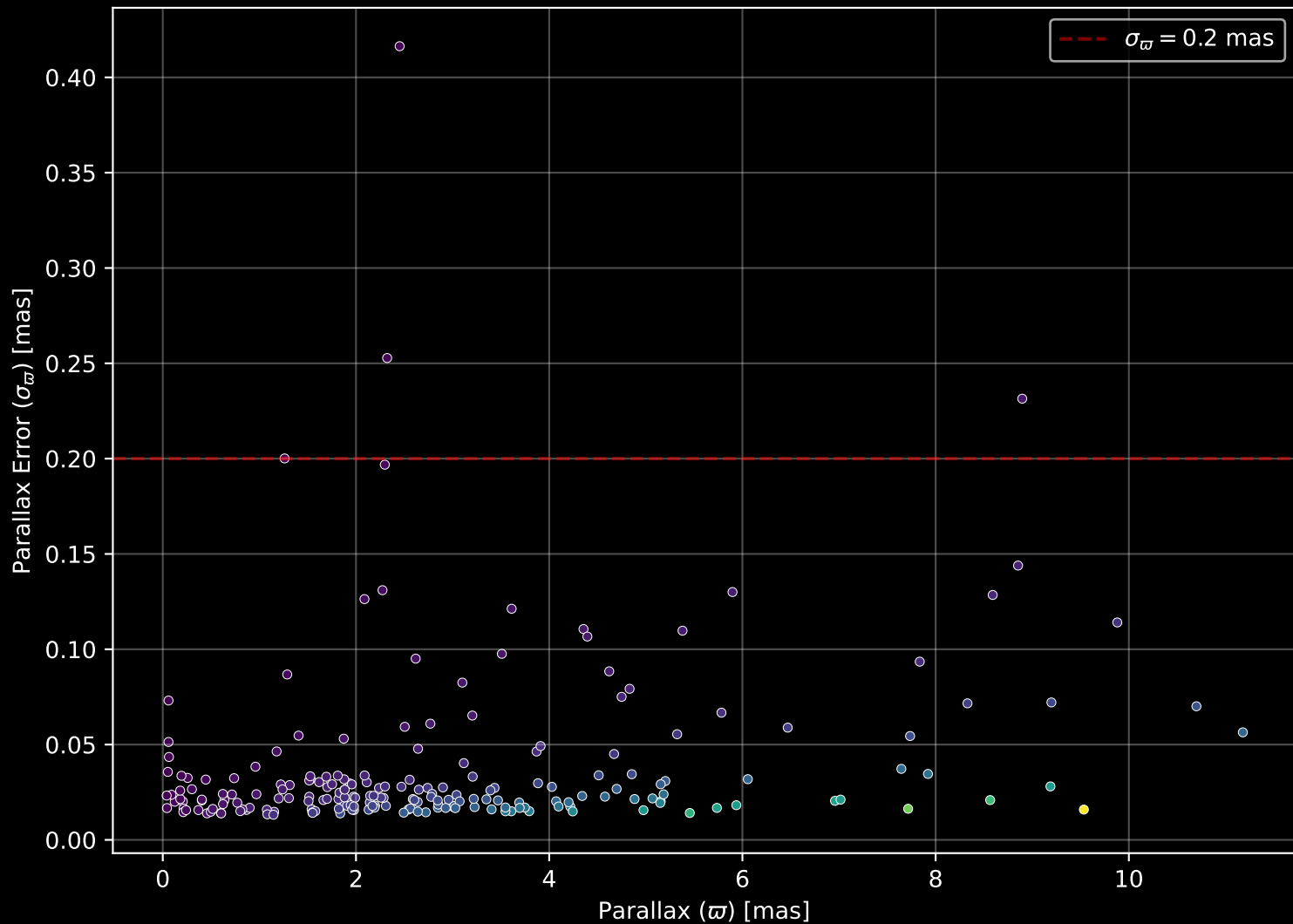
APOGEE DR17 Field: [K2_C14_251+55] Parallax Quality (n= 211)
